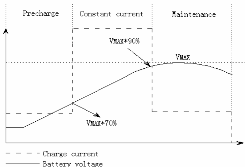
Figure 3 Typical Charging Profile
