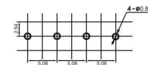
接线图 (底视图) Wiring diagram (Bottom view)
