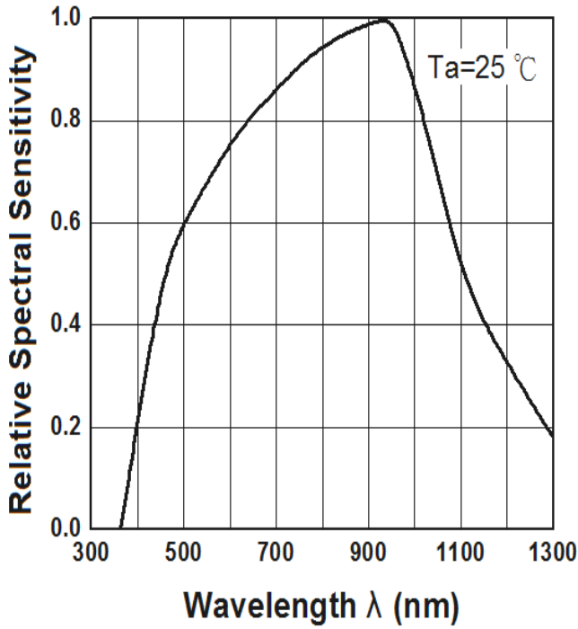
Fig.1 Spectral Sensitivity
